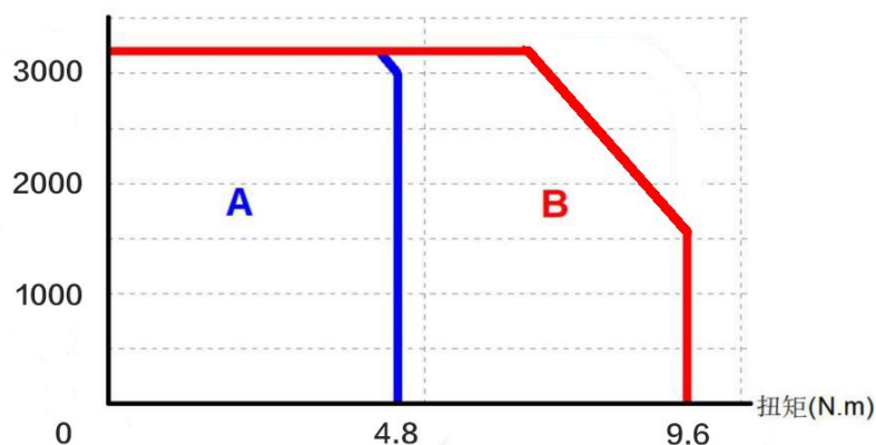
转矩—转速特性/TORQUE-SPEED CHARACTERISTICS
