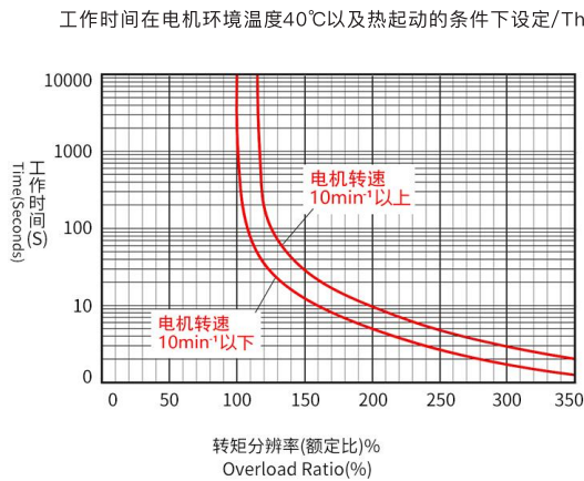
过载特性曲线/OVERLOAD CHARACTERISTICS
