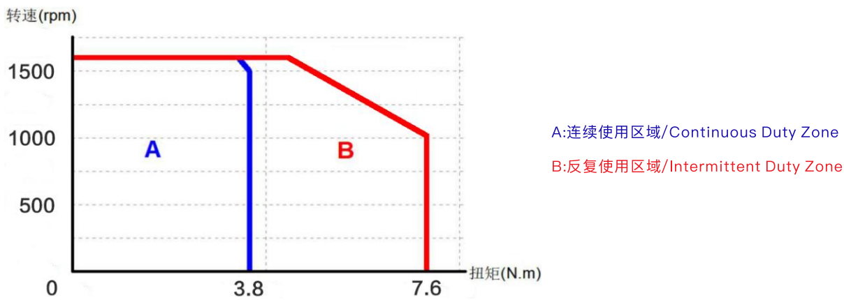
转矩—转速特性/TORQUE-SPEED CHARACTERISTICS
