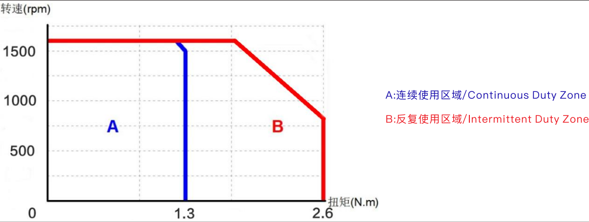
转矩—转速特性/TORQUE-SPEED CHARACTERISTICS
