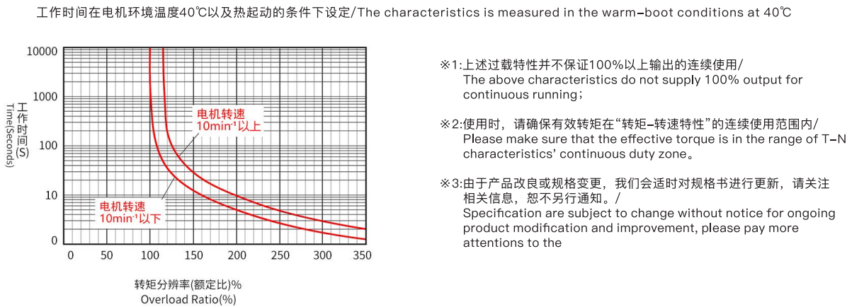
过载特性曲线/OVERLOAD CHARACTERISTICS
