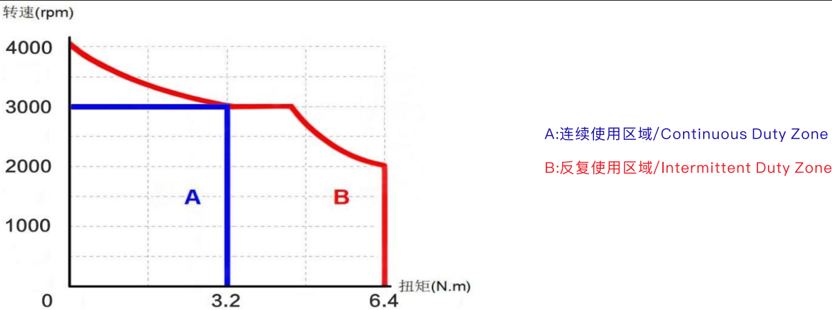
转矩—转速特性/TORQUE-SPEED CHARACTERISTICS
