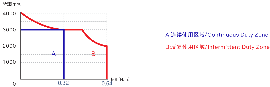
转矩—转速特性/TORQUE-SPEED CHARACTERISTICS
