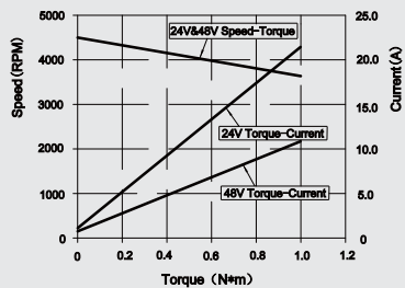
Torque-Speed- Current
