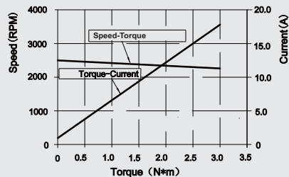
Torque-Speed- Current
