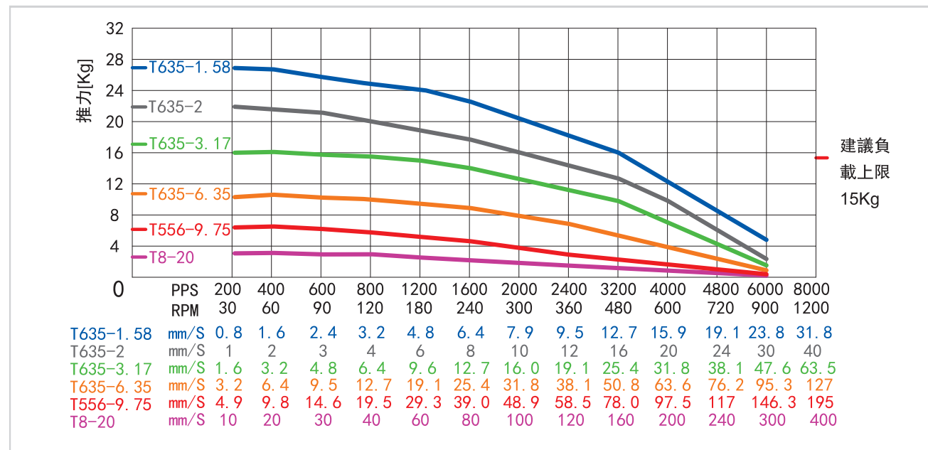
Force-Velocity Curve-17HS34
