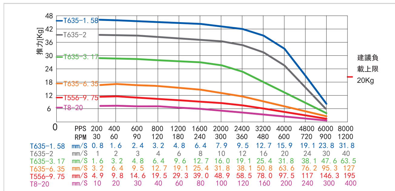
Force-Velocity Curve-17HS48
